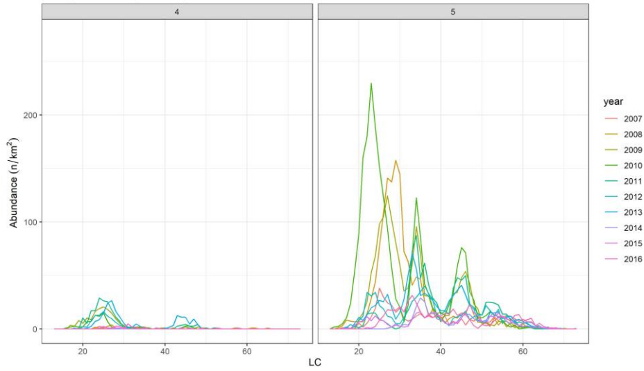
LFD (Combined by stratum)
