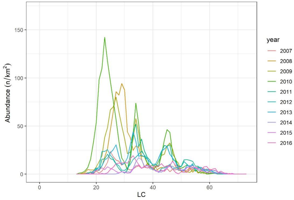
LFD (Combined by stratum)
